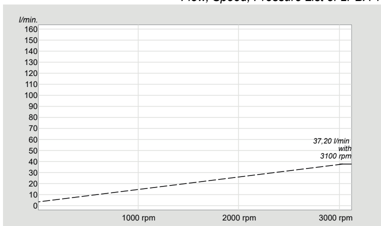
Flow, Speed, Pressure List of 2PBA 12
