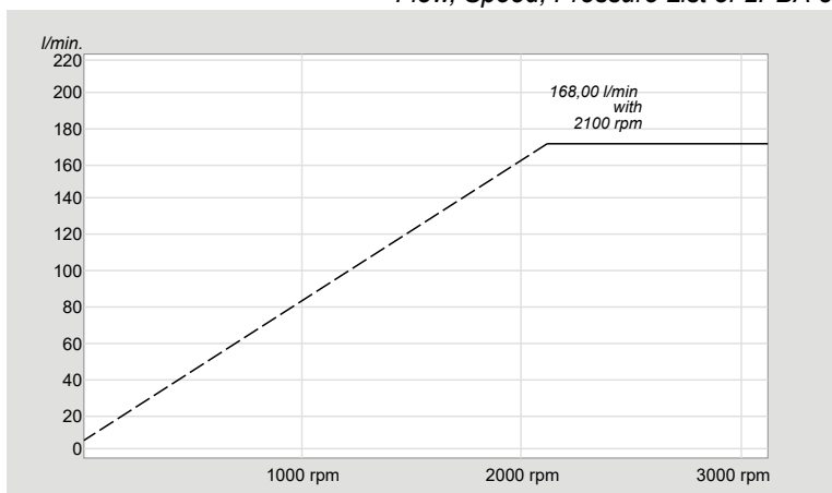
Flow, Speed, Pressure List of 2PBA 80
