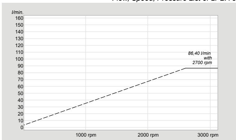
Flow, Speed, Pressure List of 2PBA 32
