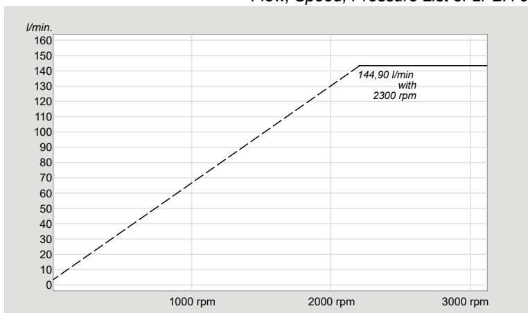
Flow, Speed, Pressure List of 2PBA 63
