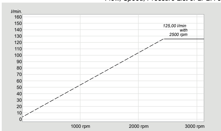
Flow, Speed, Pressure List of 2PBA 50
