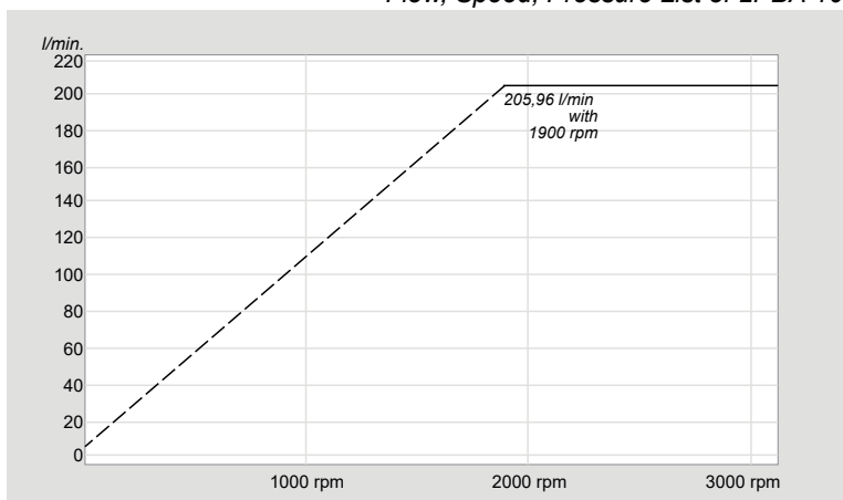
Flow, Speed, Pressure List of 2PBA 108
