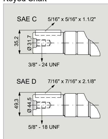
Keyed Shaft
