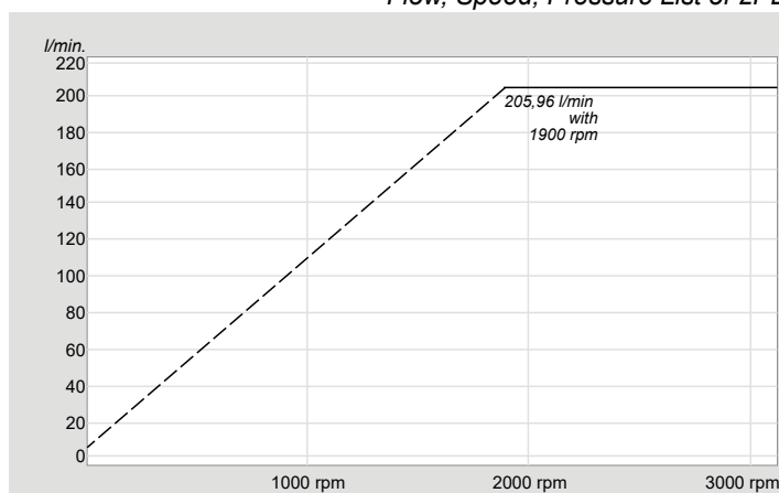
Flow, Speed, Pressure List of 2PE 108
