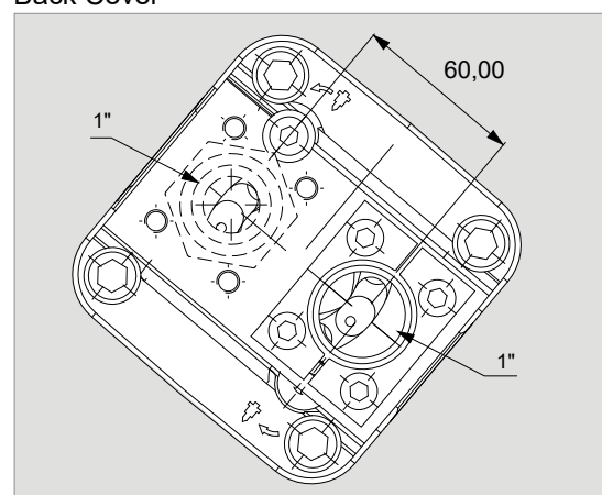
Back Cover
