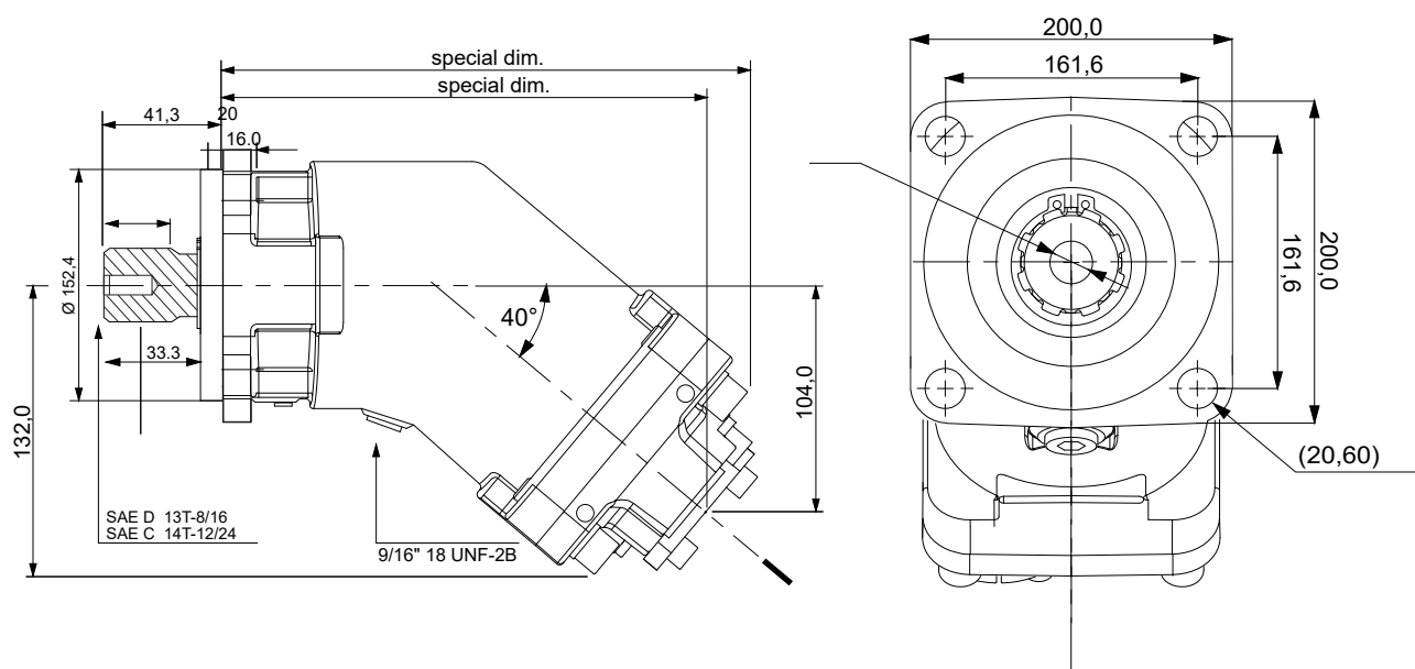
Spline Shaft
