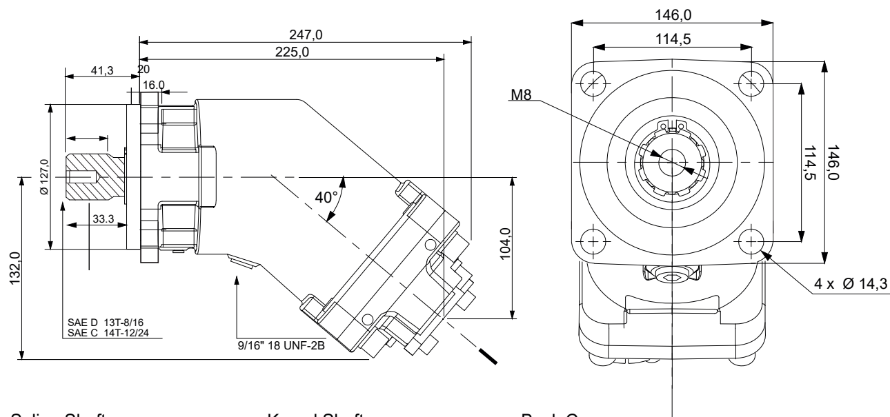
Spline Shaft
