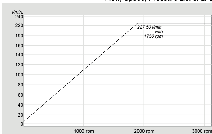
Flow, Speed, Pressure List of 2PE 130
