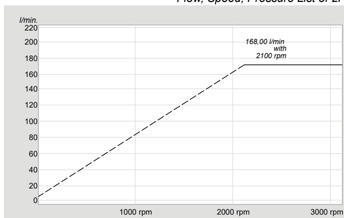
Flow, Speed, Pressure List of 2PE 80
